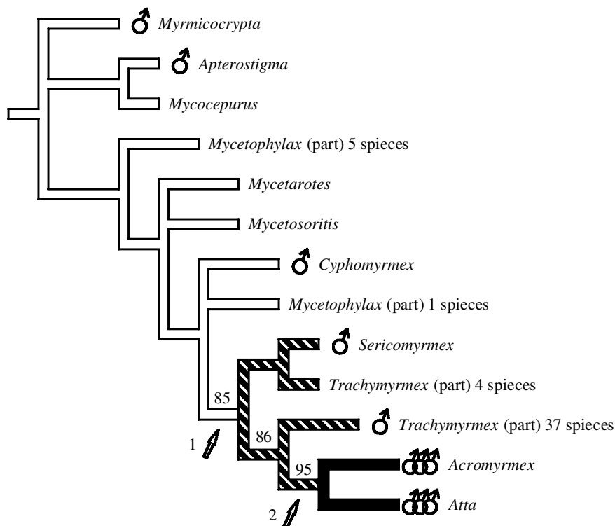
Figure 2. A simplified attine phylogeny based on Schultz (2000) and T. R. Schultz (unpublished data); see also Schultz & Meier (1995) and Wetterer et al. (1998). Numbers above branches are bootstrap values from maximum-likelihood analyses of DNA sequences from CO1 and EF-1 \alpha using the model GTR + I + gamma (see text). (White branches, lower attines; shaded branches, higher attines; black branches, leafcutter ants; single male sign, single mating; three male signs, multiple mating; arrow, possible origin of multiple mating.) The two mutually exclusive hypotheses for the transition from single to multiple queen mating tested in the present study are indicated by the arrows: (i) a hypothetical transition that occurred prior to, or coincident with, the origin of the higher attines; and (ii) a hypothetical transition that coincided with the origin of the leafcutter clade, which may include one or a few species currently still assigned to the paraphyletic genus Trachymyrmex . The results of the present study confirm the second hypothesis. See text for further details.
